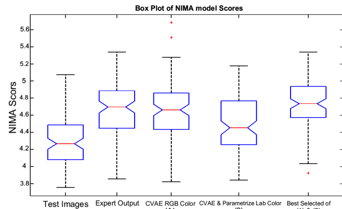
Fig. 3: The box-plot of NIMA scores of test data. Our method (the better of methods 1&2) outperforms the expert-based enhancement on 100 test images of the MIT-Adobe FiveK dataset [1].
